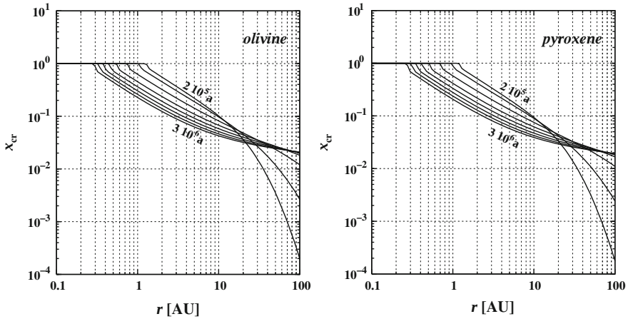
Fig. 29 Radial and temporal variation of the degree of crystallisation x_{cr} of olivine and pyroxene grains due to annealing and radial mixing of crystallized grains for a time dependent disk model. Snapshots at 2 \times 10^5 , 5 \times 10^5 , and between 1 \times 10^6 and 3 \times 10^6 year in steps of 0.5 \times 10^6 year. According to the model calculation crystalline dust is mixed into fairly distant outer regions of the disk during its evolution
