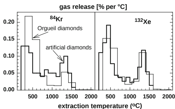
Fig. 13 Differential release upon vacuum pyrolysis of krypton and xenon from diamonds extracted from the Orgueil meteorite [23] compared with the release of gases implanted into artificial terrestrial nano-diamonds [158]. The agreement can be used to construct a history for the interstellar diamonds [158]
