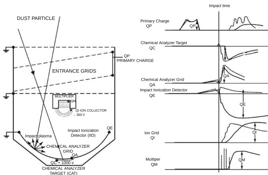
Fig. 3 The impact ionization dust analyzer aboard Cassini [14]. The left hand side of the figure show the schematics of the detector, the right hand side shows the different channels of measured signals: The particle velocity is estimated through the sequence of charges that are induced in a system of tilted entrance grids (denoted as primary charge QP on the right hand side of the figure) before they impact onto the target plate. The produced ions and electrons are detected at the target plate (QE, QA, QC) and in the ion collector (QI). Ions that are produced are accelerated due to the applied voltage and measured as a function of their flight time at a multichannelplate (QM)
