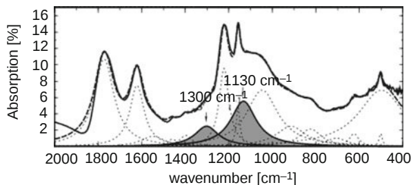
Fig. 11 IR absorption spectra measured on a sample of diamond extracted from the Murchison meteorite. The absorption expected due to nitrogen as single atoms in the diamonds (gray area) – probably the only signatures independent from chemical history and current environment – may be present, but are masked by the presence of much larger peaks due to attached surface groups. Figure provided by A. Braatz [146]
