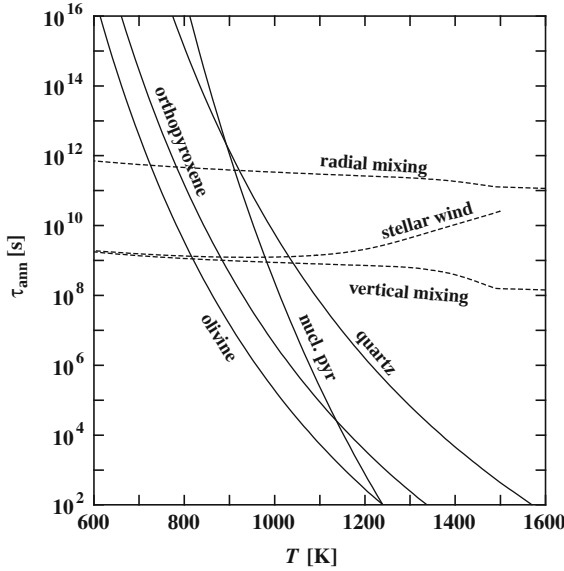
Fig. 12 Characteristic time scales for annealing of a 0.1 μm dust grain and time required for formation of growth centres (nucleation) in enstatite ( Full lines ). Data for the activation energy from Fabian et al. [92]. For comparison, the time scales for radial and vertical transport processes (mixing) in protoplanetary discs and the hydrodynamic timescale r/v for a stationary stellar wind model are shown as dashed lines
