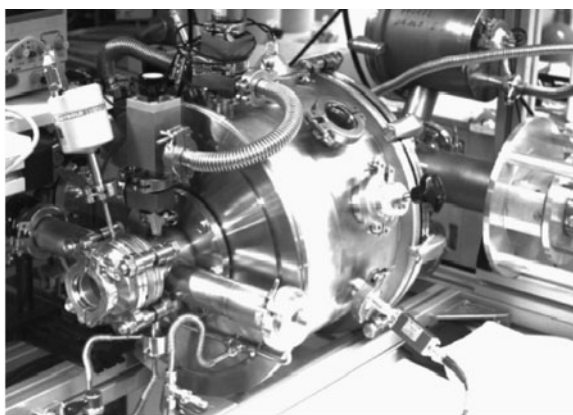
Fig. 1 Jena laser pyrolysis system for the production of small particles
