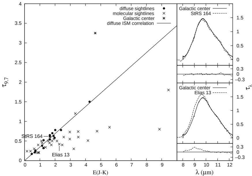
Fig. 14 Comparison of near-IR extinction and optical depth in the 9.7\ \mu\text{m} amorphous silicate band for different lines of sight in the galaxy. The right-hand panels show (i) the normalized silicate band shapes towards the galactic center and the diffuse ISM line of sight towards the background star StRS 164 ( upper right ) and the difference between these two band shapes; and (ii) the molecular cloud line of sight Elias 13 ( lower right ) and the galactic center, and their difference. Figure adapted from van Breemen et al. (in preparation)
