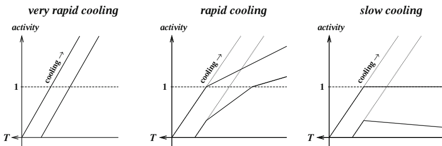
Fig. 19 Schematic evolution of the activities of two competing substances that can be formed from the same gas phase material during cooling. Left : Cooling is so rapid that essentially no condensation occurs. Middle : Rapid cooling where the more stable substance has not consumed the condensable material at the instant where the less stable material starts to condense. Right : Cooling is so slow that the system always is close to chemical equilibrium. The less stable material never condenses because its activity always remains < 1
