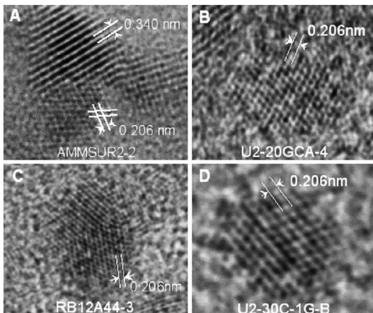
Fig. 7 Lattice-fringe images of nano-diamonds (0.206 nm spacings) in Antarctica micrometeorite AMMSRU2-2 and IDPs U2-20-GCA, RB12A44, and U2-30C-1G-B. See [85]
