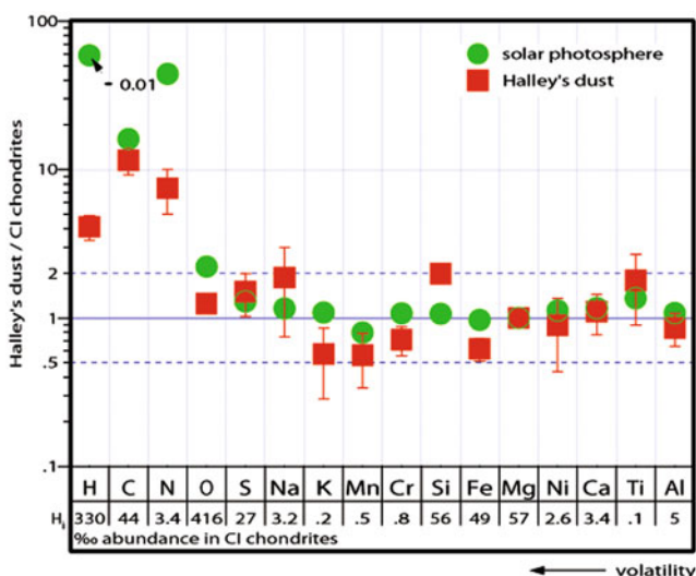
Fig. 6 \text{Mg}=1 normalized element abundances in the dust of comet Halley and the solar photosphere, both relative to the abundances in CI-chondrites. The elements are ordered according to their volatility and recent abundance values were used as explained in the text. The solar hydrogen abundance is multiplied by 0.01. Because of the lack of calibration, Halley's dust data are believed to be certain within a factor two
