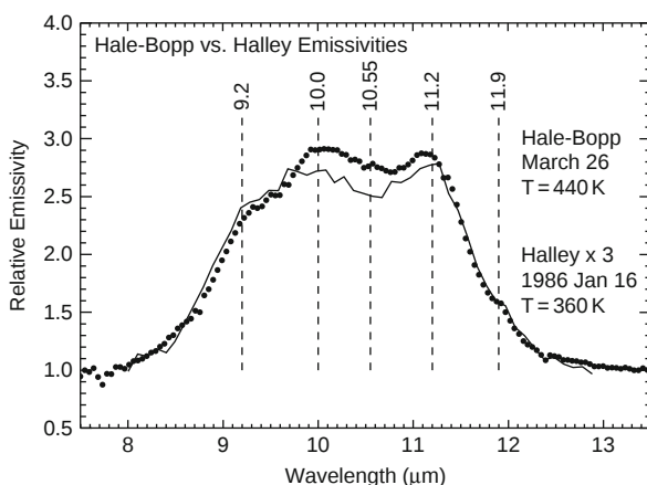
Fig. 3 The silicate feature in Hale-Bopp ( filled circles ) [27] and P/Halley ( line ) [23]. Each spectrum has been divided by a blackbody at the temperature shown and the Halley spectrum has been multiplied by 3. ( from [27])
