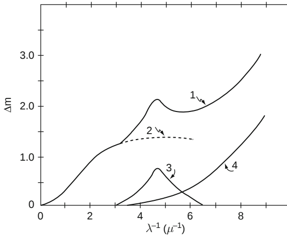
Fig. 6 The decomposition of the extinction curve ( I ) in three partial curves responsible for the visual and NIR extinction (2), the superimposed UV band (3) and the FUV extinction (4). After [131]
