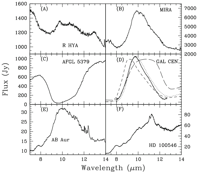
Fig. 4 Examples of 10\text{ }\mu\text{m} amorphous silicate band shapes in different astronomical environments. (a) R Hya, a low mass loss AGB star with a 10\text{ }\mu\text{m} band dominated by simple oxides and a minor amorphous silicate contribution, (b) Mira, an AGB star showing a strong amorphous silicate band very similar in shape to that seen in the ISM, (c) the OH/IR star AFGL 5379, an AGB star with very high mass loss rate showing a strong amorphous silicate absorption, (d) the galactic centre 10\text{ }\mu\text{m} silicate band shape ( solid line ) which is observed in absorption, but shown in emission here to illustrate the band shape, and compared to laboratory samples of 0.1 and 2\text{ }\mu\text{m} amorphous olivines ( dotted and long-dashed lines , respectively) and small pyroxene grains ( short dashed line ), (e) the Herbig Ae/Be star AB Aur, and (f) the Herbig Ae/Be star HD 100546, whose silicate band shows prominent contributions from polycyclic aromatic hydrocarbons and from crystalline silicates
