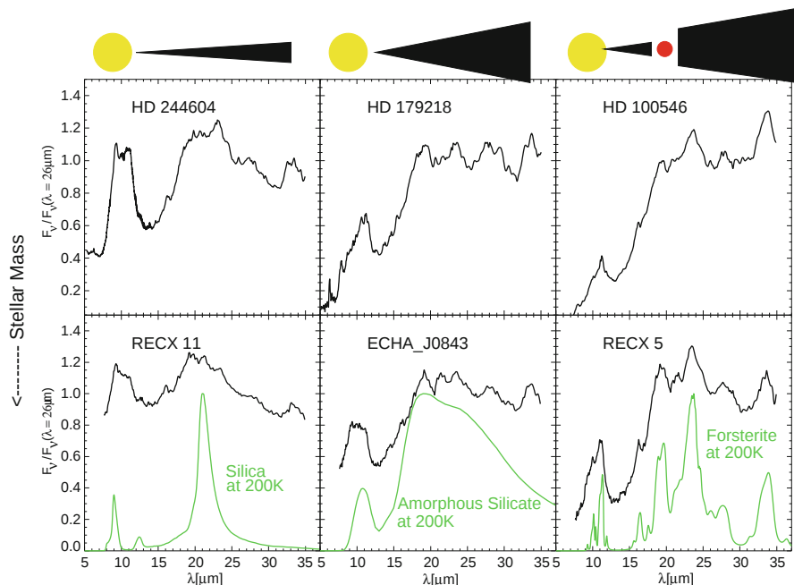
Fig. 16 Spitzer IRS spectra of proto-planetary disks surrounding young stars. The top row panels are intermediate mass ( 2\text{--}3\,M_{\odot} ) Herbig Ae/Be stars (Juhász et al. [294]), while the bottom row are those of low mass stars in the 8 million years old \eta Cha cluster ( 0.7 , 0.2 and 0.2\,M_{\odot} for RECX11, ECHA-J0843 and RECX5, respectively, [239, 240]. The pictographs on top show a possible geometry of the disks plotted in the different columns. Also shown are the dust opacities of silica, amorphous silicate and forsterite at 200 K. The strong 33.6\,\mu\text{m} forsterite band indicates the presence of cold crystalline silicate, indicative of substantial processing at large distance from the star. This process occurs in disks surrounding stars with a wide range of mass
