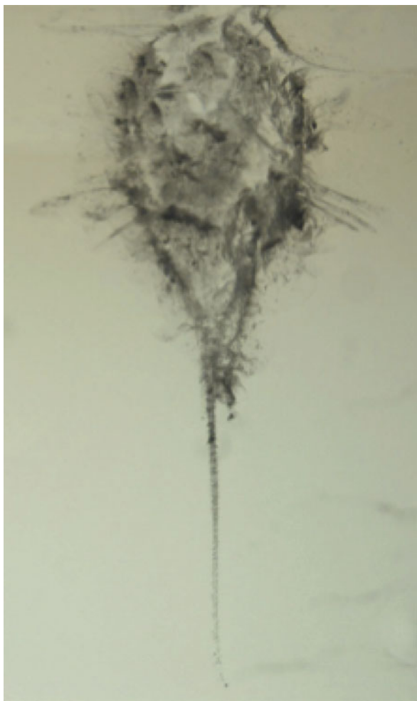
Fig. 5 Example of a track (C054-T3) in the Wild 2 aerogel collector. showing bulbous upper cavity with narrow tracks of terminal grains branching from it
